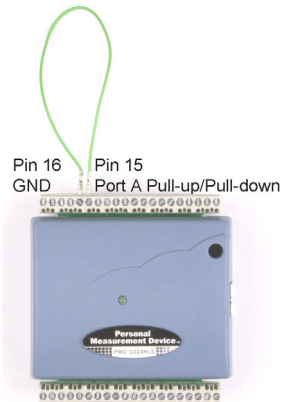
Figure 3-6. Pull-down connection for Port A
